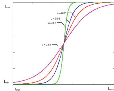
Figure 1: Non linear ACE or adaptive contrast enhancement curve. Acting as an inverse normalized optical modulation transfer function (MTF, see http://www.microscopyu.com/articles/optics/mtfintro.html ) correcting optical coherence factor (OCF) or relationship between NA of detector (CCD) and the objective \gamma = \text{NA}_{\text{ccd}}/\text{NA}_{\text{obj}} .
